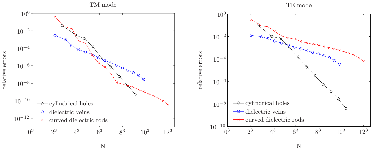
Fig. 11. The convergence of the relative error of the smallest TM ( left ) and TE eigenvalue ( right ) at k_c for the crystals with cylindrical holes, with dielectric veins and with inversely curved rods (Fig. 7, same geometric and dielectric parameters as in Fig. 8 and Fig. 9 ( left )). The computations were done with p -FEM.
