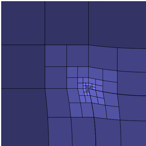
Fig. 4. The mesh is refined towards the interface corners, while the polynomial order increases linearly away from material corners. In this example the mesh is 2-irregular, however we can cope with arbitrarily irregular meshes.
