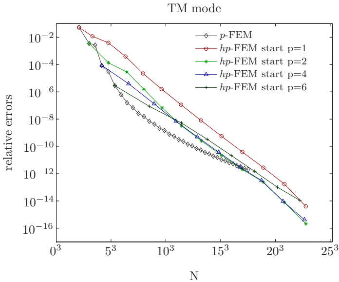
Fig. 13. Convergence of the relative error of the first eigenvalue at k_c for the TM-mode (left) and TE mode (right) of the crystal with curved dielectric veins (the third crystal in figure 7). We use \varepsilon = 100 in the white region and \varepsilon = 1 in the rest. The distance between the corners is 0.6a , the circles used for the veins have radius 0.8a , their midpoints lie on the perpendicular bisectors of the sides. We use p -FEM and hp -FEM, the latter with different initial polynomial degree.
