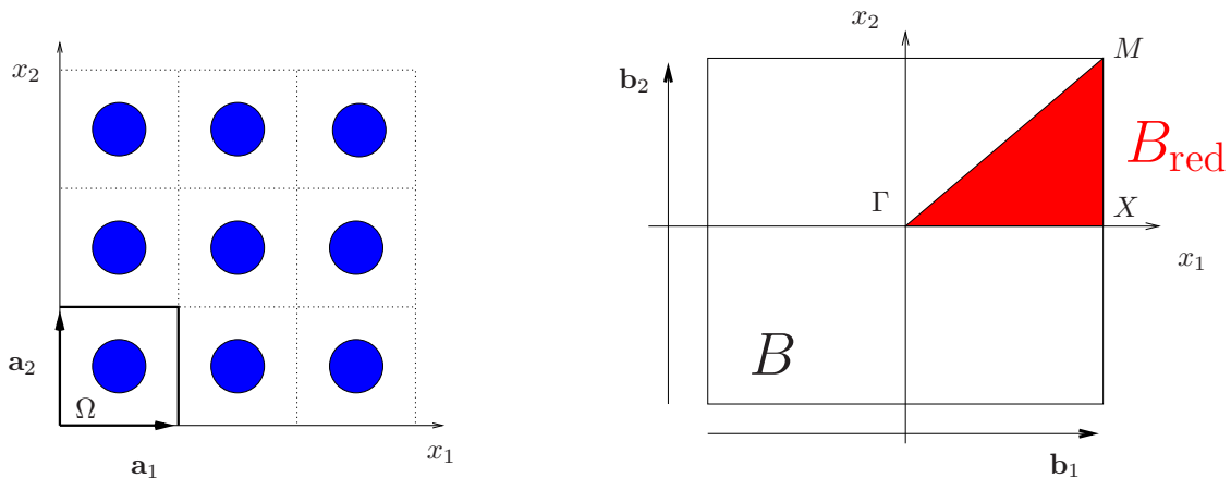
Fig. 2. The left picture shows a two dimensional setting with periodicity domain \Omega . On the right side we see the corresponding Brillouin zone B and the reduced Brillouin zone B_{\text{red}} (red triangle).
