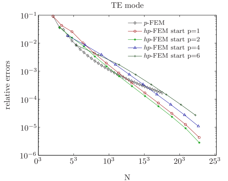
Fig. 13. Convergence of the relative error of the first eigenvalue at k_c for the TM-mode (left) and TE mode (right) of the crystal with curved dielectric veins (the third crystal in figure 7). We use \varepsilon = 100 in the white region and \varepsilon = 1 in the rest. The distance between the corners is 0.6a , the circles used for the veins have radius 0.8a , their midpoints lie on the perpendicular bisectors of the sides. We use p -FEM and hp -FEM, the latter with different initial polynomial degree.
