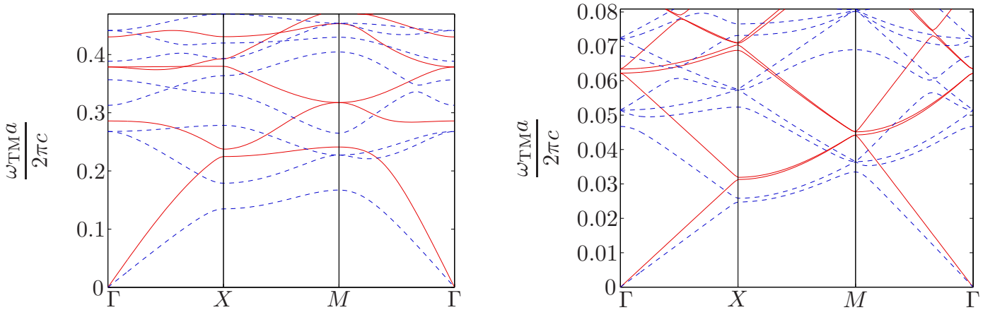
Fig. 9. Band structure of the crystal with inversely curved dielectric rods with radius 0.8 a (midpoints on the perpendicular bisectors of the sides) and distance between corners of 0.9 a ( left ) and of the crystal with a 9 \times 9 structure of dielectric veins of thickness 0.1 a/9 ( right ). The dielectric medium (dark in figure 7) has \varepsilon = 20 , in the rest of the structure we have \varepsilon = 1 . Solid lines denote the TE modes, dashed lines denote the TM modes.
