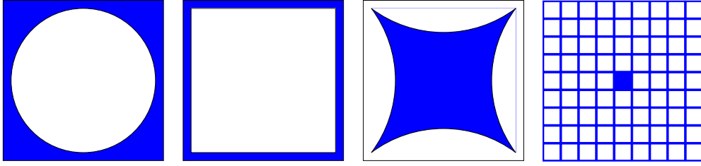
Fig. 7. The elementary cell with cylindrical holes ( left ), that with dielectric veins ( inner left ), that with inversely curved dielectric rods ( inner right ) and that with a 9 \times 9 structure of dielectric veins with a periodic defect in the middle ( right ). The white region is air ( \varepsilon = 1 ), the blue region is a dielectric medium ( \varepsilon > 1 ).
