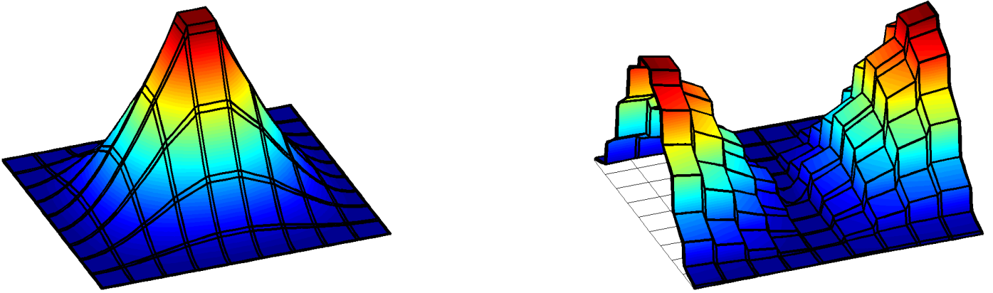
Fig. 10. Squared amplitude of the first TM eigenfunction |e_{\mathbf{k}}(\mathbf{x})|^2 (left) and TE eigenfunction |h_{\mathbf{k}}(\mathbf{x})|^2 (right) at the M point of the crystal with a 9 \times 9 structure of dielectric veins of thickness 0.1a/9 . The dielectric medium (dark in figure 7) has \varepsilon = 20 , in the rest of the structure we have \varepsilon = 1 . As the TE eigenvalue is twofold, there is another eigenfunction, which results from an interchange of x_1 and x_2 .
