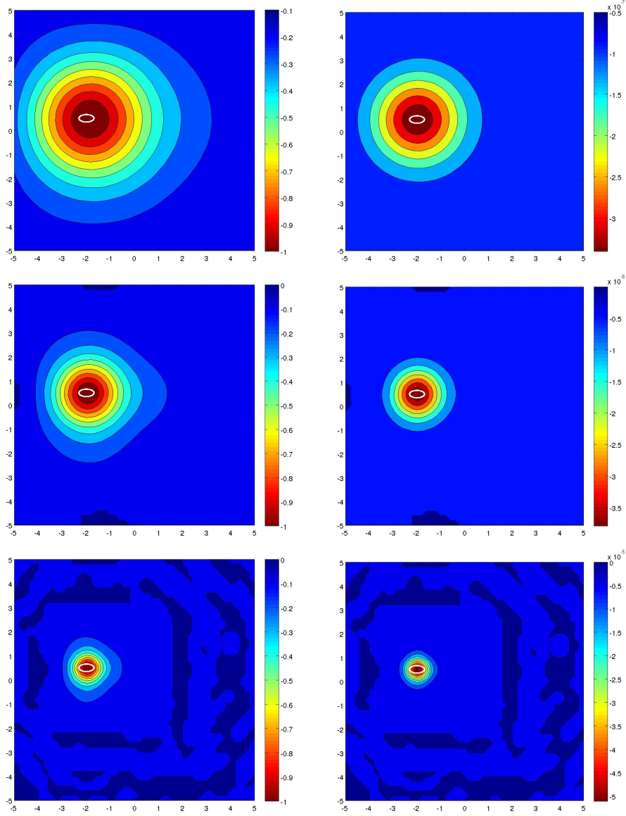
Figure 3. Contour plots of z \mapsto \mathcal{T}_3(z) (left column) and z \mapsto \hat{J}_6(z) (right column) in the horizontal plane containing the true obstacle center \hat{x} , for obstacle (B), testing configuration 5 \times 5 and noise-free data. Testing frequencies are kd = 1 (top row), kd = 2 (middle row) and kd = 5 (bottom row).
