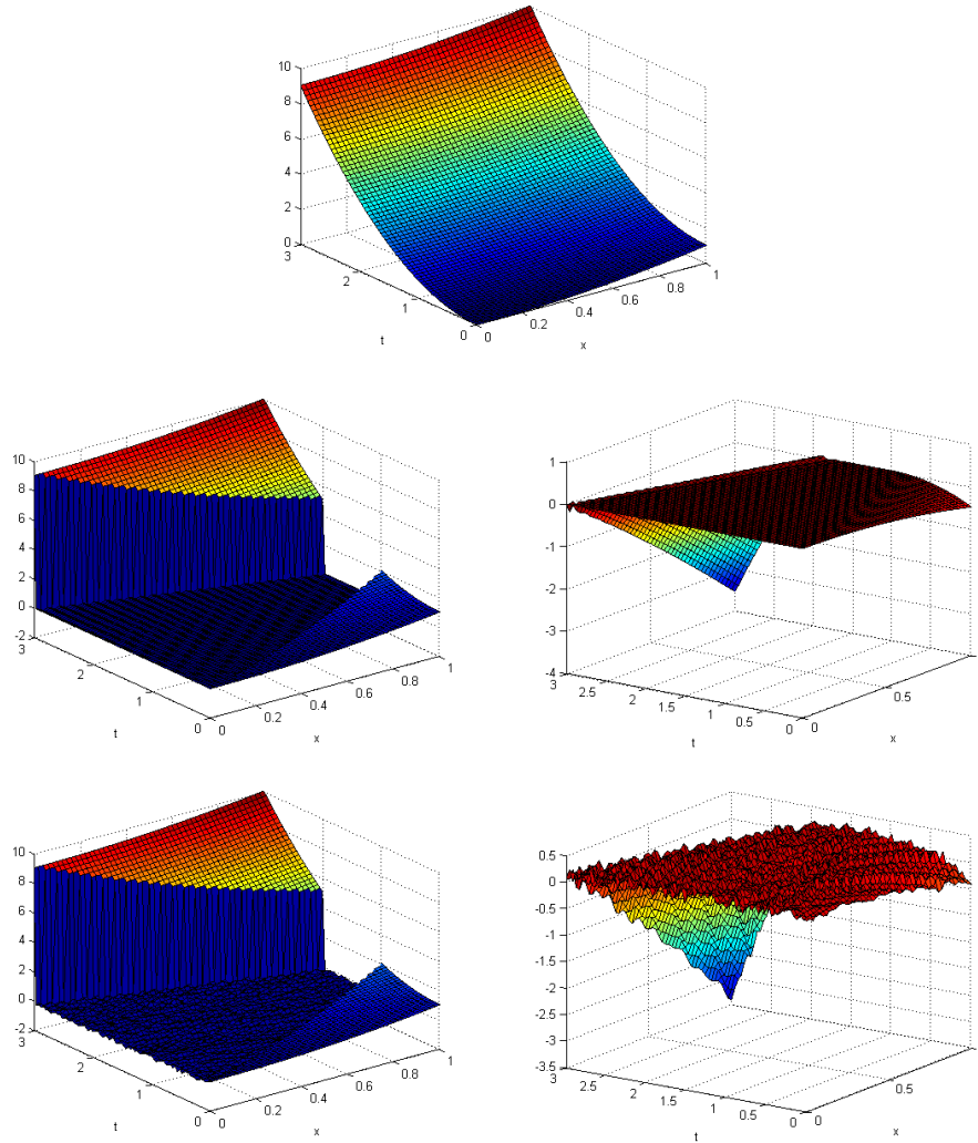
FIGURE 11. Impact of the amplitude of noise. Top: exact solution u . Middle left: discrepancy u_A - u for \sigma = 0 . Middle right: discrepancy u_{\varepsilon,\delta} - u for \sigma = 0 . Bottom left: discrepancy u_A - u for \sigma = 0.05 . Bottom right: discrepancy u_{\varepsilon,\delta} - u for \sigma = 0.05 .
