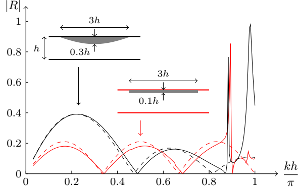
FIG. 6. Plane wave reflection coefficient of a waveguide segment with a discontinuous narrowing, and a smooth, sine shaped, narrowing as a function of the non dimensional frequency kh/\pi with \rho/\rho_0 = B/B_0 = 3 . Plain lines: numerical solution calculated with N = 20 modes, dashed lines: analytical solutions.
