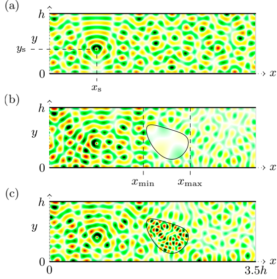
FIG. 2. Wavefield (real part) generated by a point source in a waveguide containing a scatterer with a contrast in \rho (no contrast in B ). (a) Incident wave in the empty waveguide produced by a point source, Eq. (23), with x_s = h , y_s = 0.4h . In the presence of a scatterer with contrasts (b) \rho/\rho_0 = 10 ; (c) \rho/\rho_0 = 0.3 . kh = 19.5\pi , calculations have been done using N = 30 modes (20 propagating modes).
