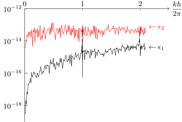
FIG. 4. Evaluation of the properties of reciprocity and energy conservation: relative errors \epsilon_1 and \epsilon_2 (Eq. 30), computed with 17 modes, as function of the non dimensional frequency kh/2\pi . Calculations have been performed for square scatterers of side a = h/10 , centered at y = h/2 , with B/B_0 = 2 , \rho/\rho_0 = 1 for an incident plane wave.
