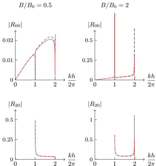
FIG. 7. Reflection coefficients R_{00} and R_{20} as a function of the non dimensional frequency kh/2\pi for a plane wave at normal incidence to a grating made of square penetrable scatterers of side h_s = h/10 , mass density \rho_0 = \rho , and a bulk modulus B_0 such that B/B_0 = 0.5 (left), B/B_0 = 2 (right). Plain lines: numerical results, dashed lines: analytical.
