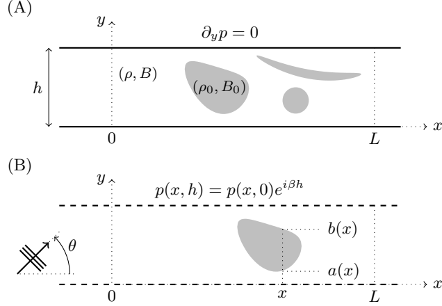
FIG. 1. Two configurations are studied. (A) The scatterers are contained in a 2D waveguide with Neumann boundary conditions at the walls. (B) An infinite periodic row of scatterers is considered.
